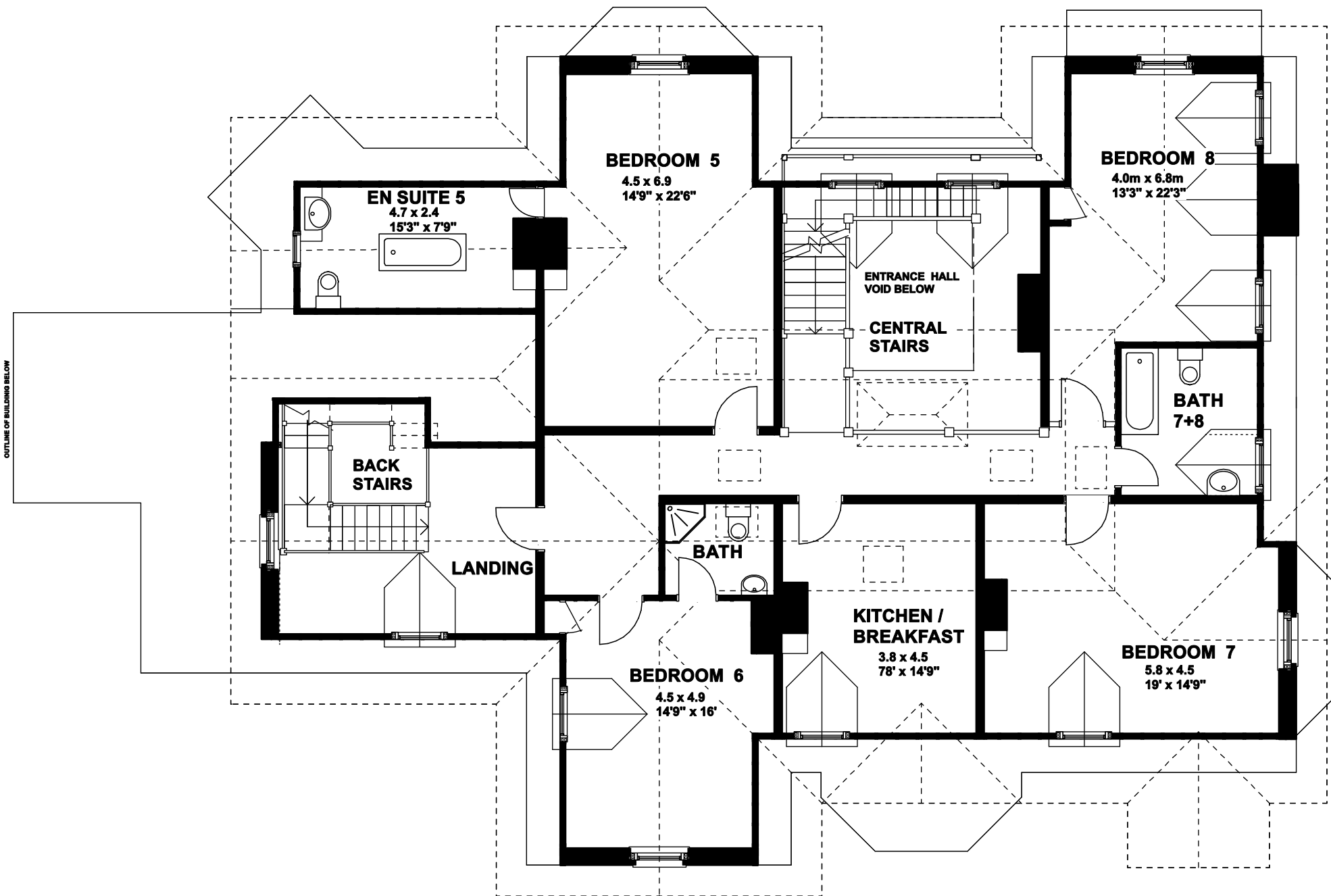
SECOND FLOOR PLAN 1:100
